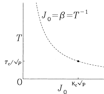
FIG. 3. The line J_0 = \beta in the phase diagram (shown dashed) on which the internal energy is obtained exactly. There is a singularity in the internal energy at the point J_0 = \beta = \sqrt{p}K_c indicated on the line, implying a phase transition.
